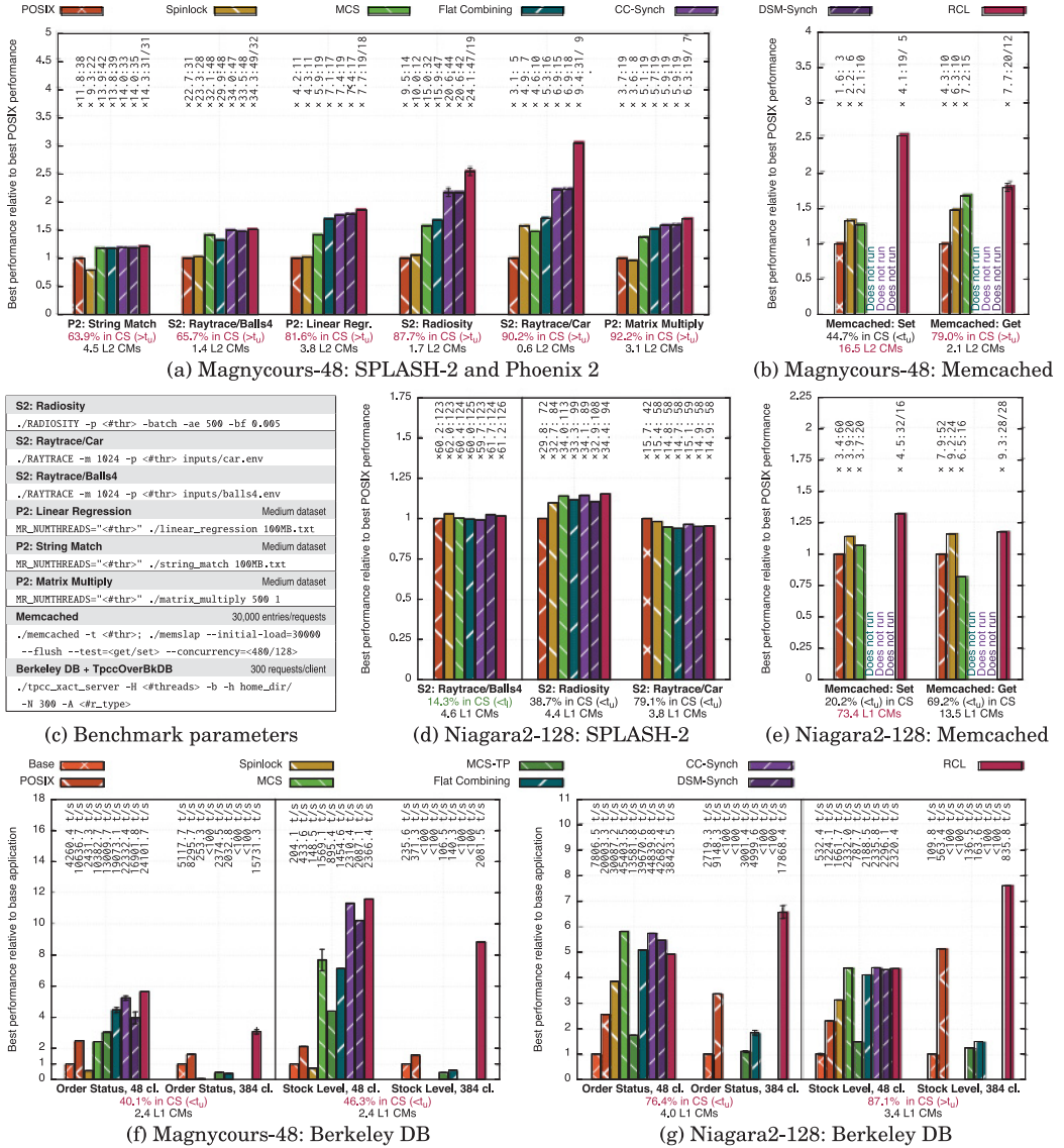
Five runs per data point, error bars show standard deviation when relative standard deviation is > 5\% . In this figure, t_l and t_u stand for the lower and the upper threshold corresponding to each experiment.
