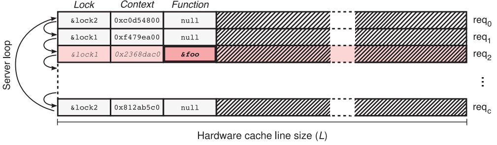
Fig. 1. The request array.
