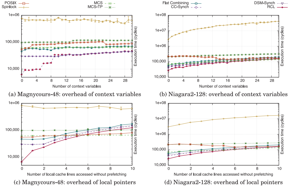
Fig. 19. Overhead of context variables and local pointers.
