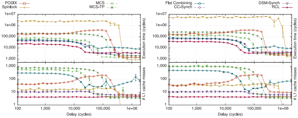
(a) One shared cache line per CS (b) Five shared cache lines per CS Five runs per data point, error bars show standard deviation when relative standard deviation is > 5%.
