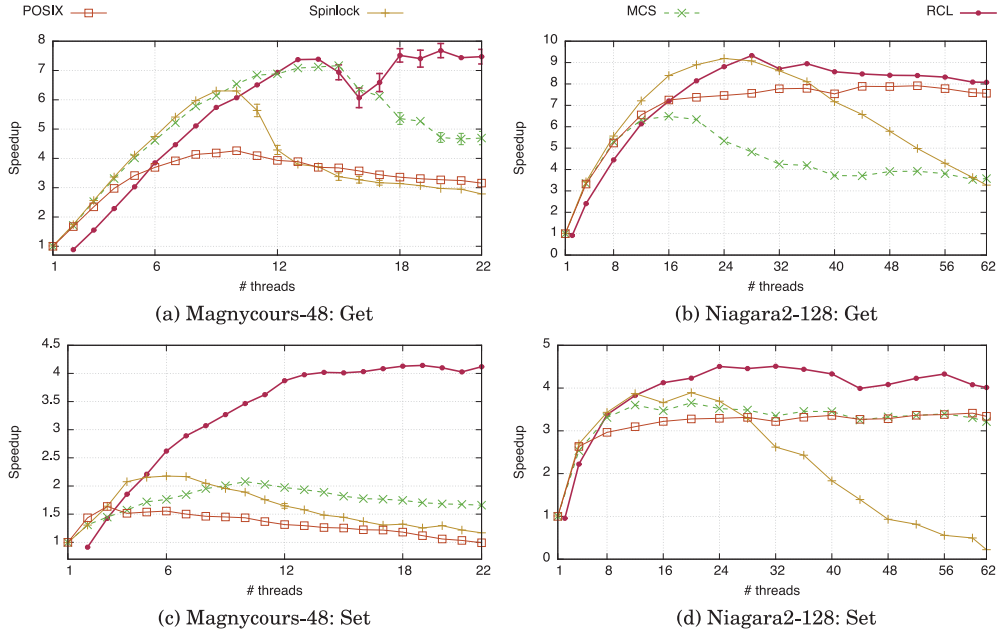
Fig. 13. Memcached speedup.
