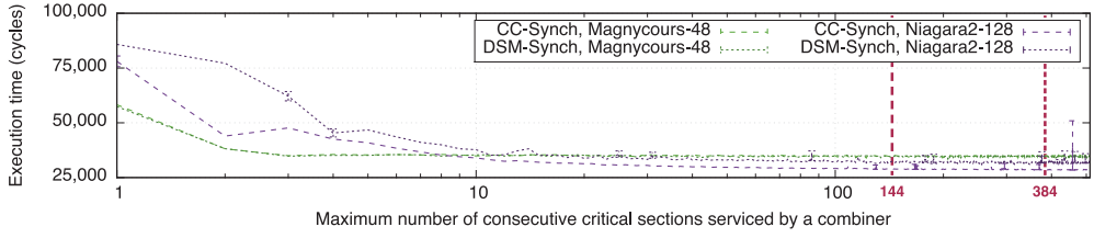
Fig. 4. Influence of MAX_COMBINER_CS on CC-Synch and DSM-Synch.
